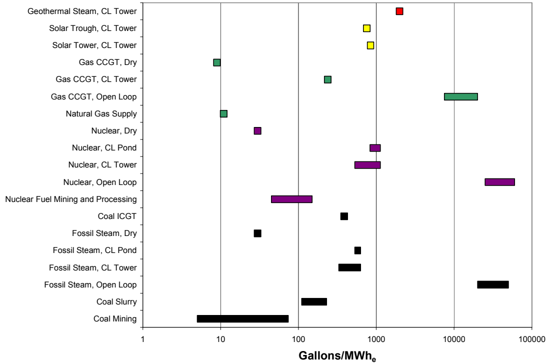
Figure V-1. Water Withdrawal for Power Generation
