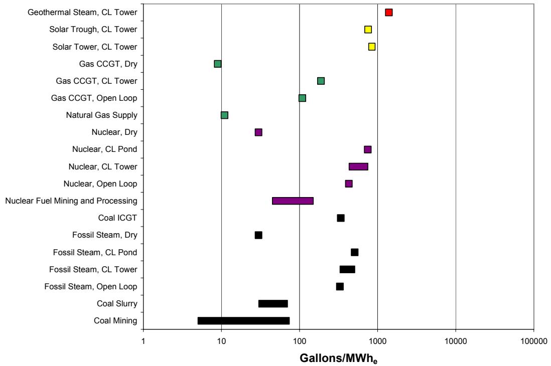
Figure V-2. Water Consumption for Power Generation
